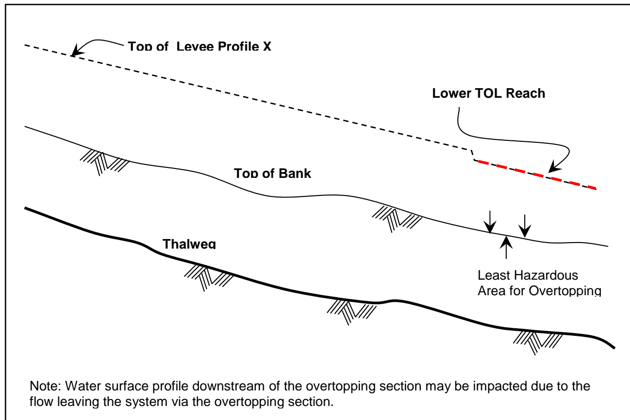
Figure 4. Final overtopping reach design.
