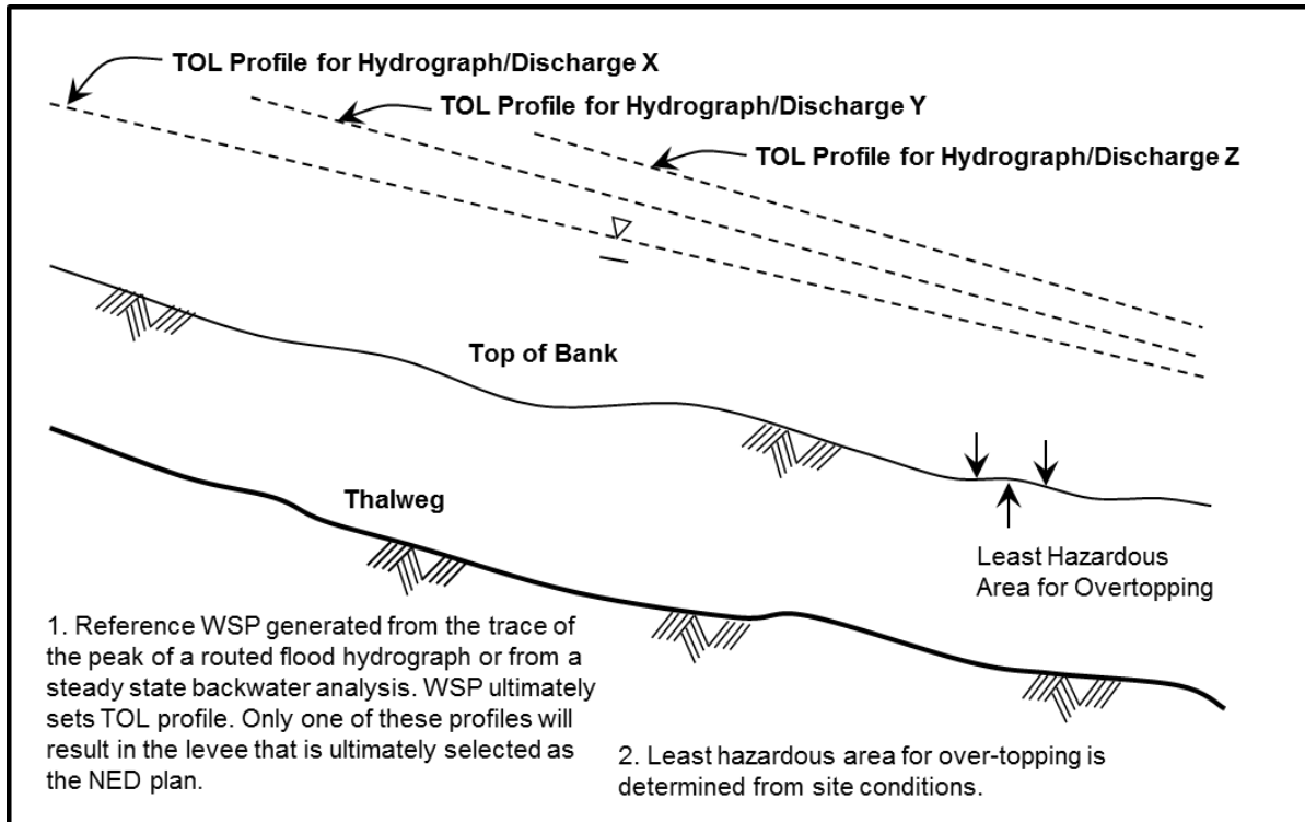
Figure 3. Pairing of profiles to each levee height.
