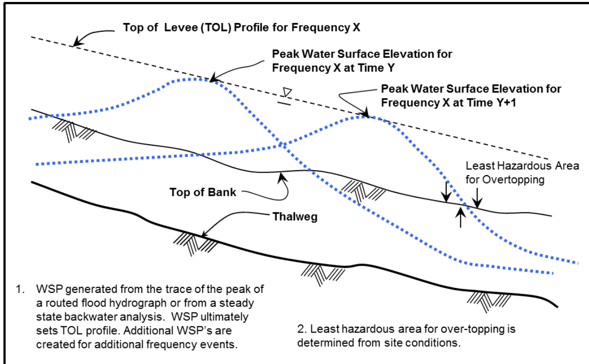
Figure 2. Top of levee (TOL) profiles
