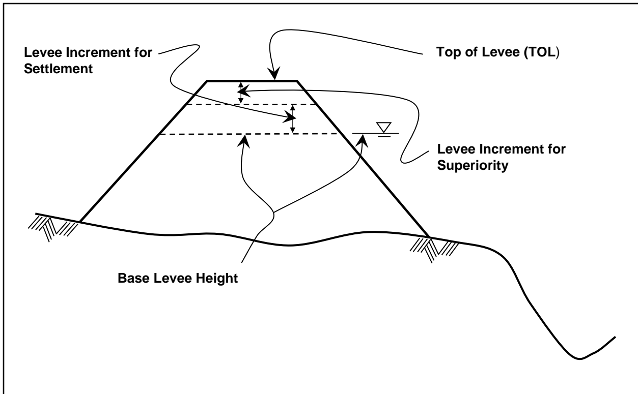
Figure 1. Arriving at Top of Levee Elevation (not all possible increments are shown)
