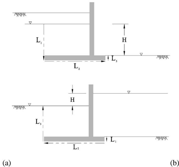
Figure 2. Seepage paths for gradient determination. H =change in total head and (seepage) path length L=L_1+L_2+L_3 . (a) Retaining wall with high head on the “retained” side of the wall. (b) Flood wall with high head on the “wet” side of the wall. Observe these vectors denote the direction of seepage.
